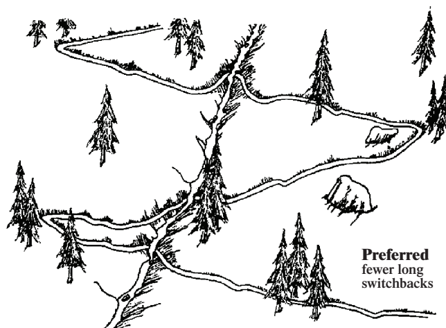
Figure 72—Long sections of trail between switchbacks are usually better than short sections—fewer switchbacks will be needed, with fewer turns to shortcut.
